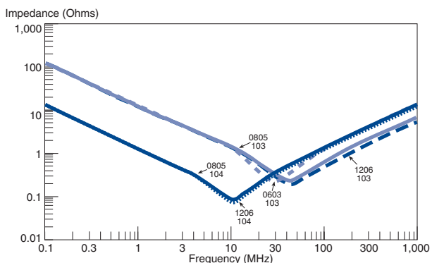
FIGURE 6. Impedance versus Frequency X7R Dielectric
